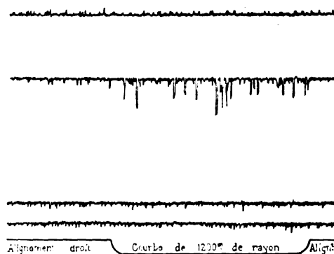
Fig. 4. Inspection Record of Track on Curve, Showing Influence of Centrifugal Force.
