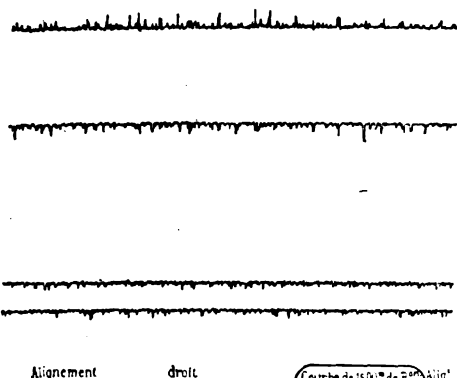
Fig. 2. Inspection Record of Well-Maintained Track.
