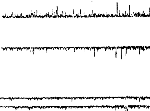
Fig. 3. Inspection Record of Track in Poor Condition.
