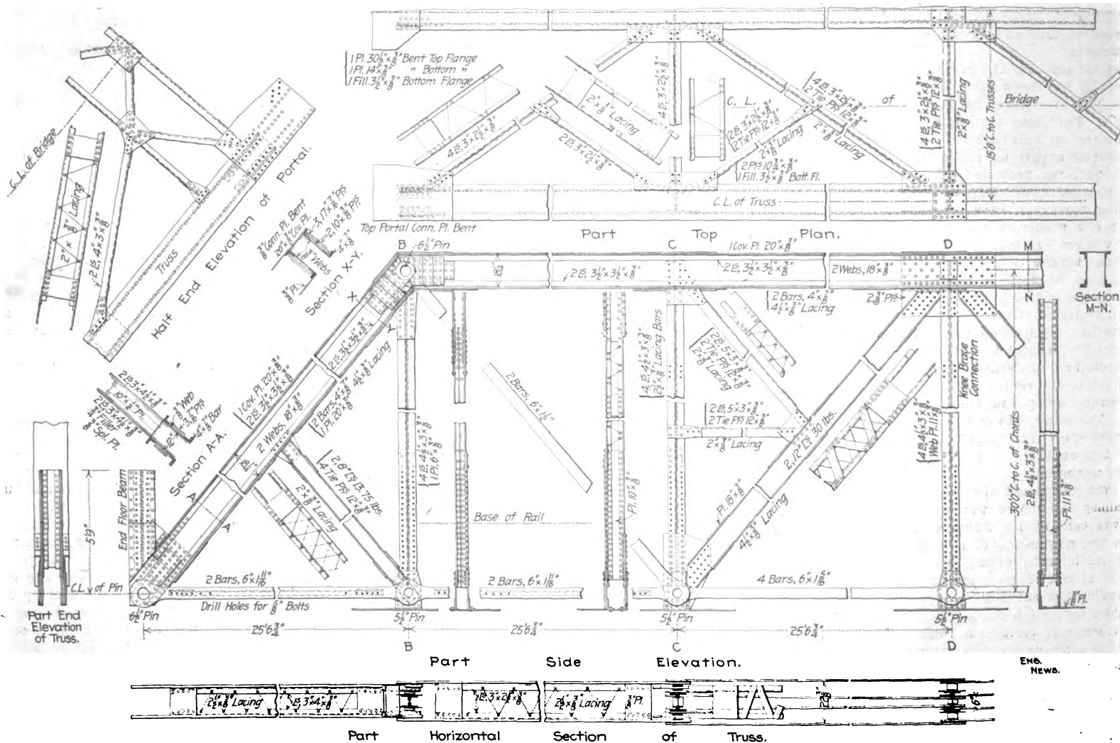
FIG. 2 HALF SIDE ELEVATION OF SCHAUB TRUSS.
